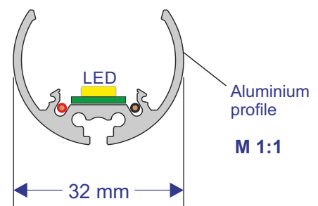
Cross-section and dimensions (For indoor installation or for outdoor installation IP65 )
