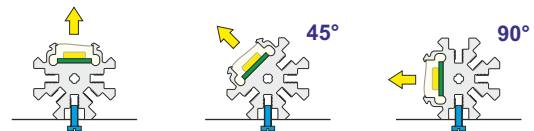
Screw mounting using the M3 longitudinal thread
