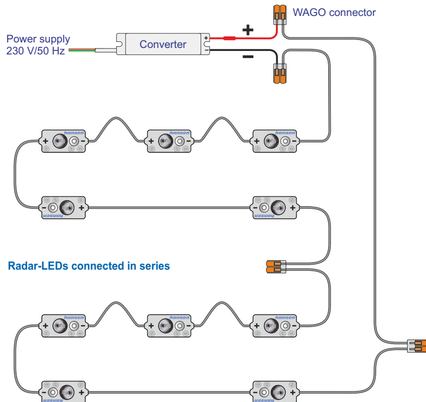
Connection example for the Radar-LED (LEDs in series connection)
