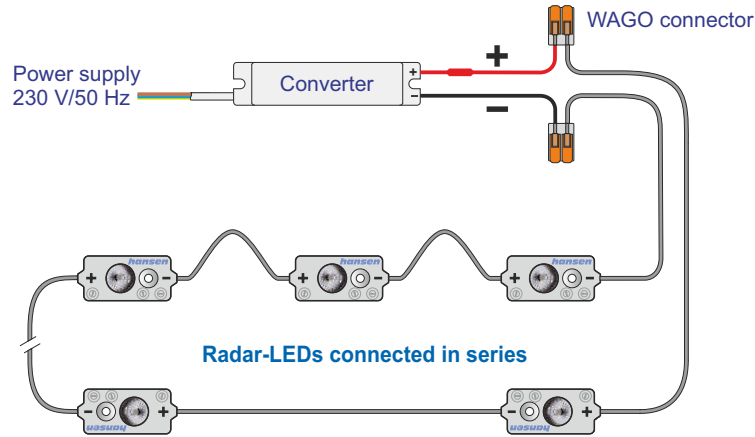
Connection example for the Radar-LED (LEDs in series connection)
